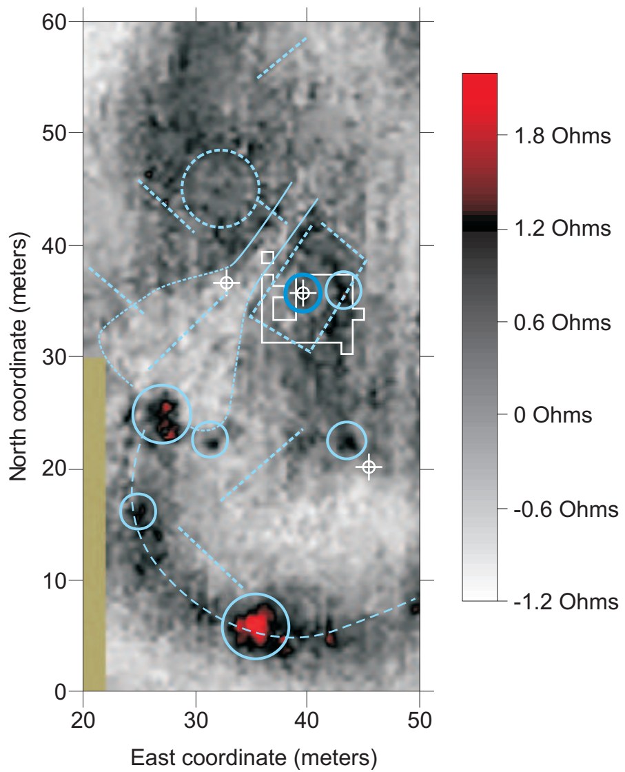
Eaststep Site resistance survey
